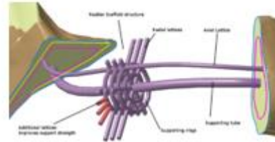
Figure 11. Rudder Scaffold structure
