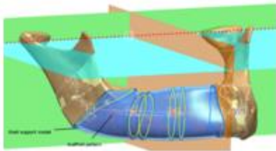
Figure 9. A shell volume model (supporting structure) together with a polygonal model of a lower jaw and the scaffold model
