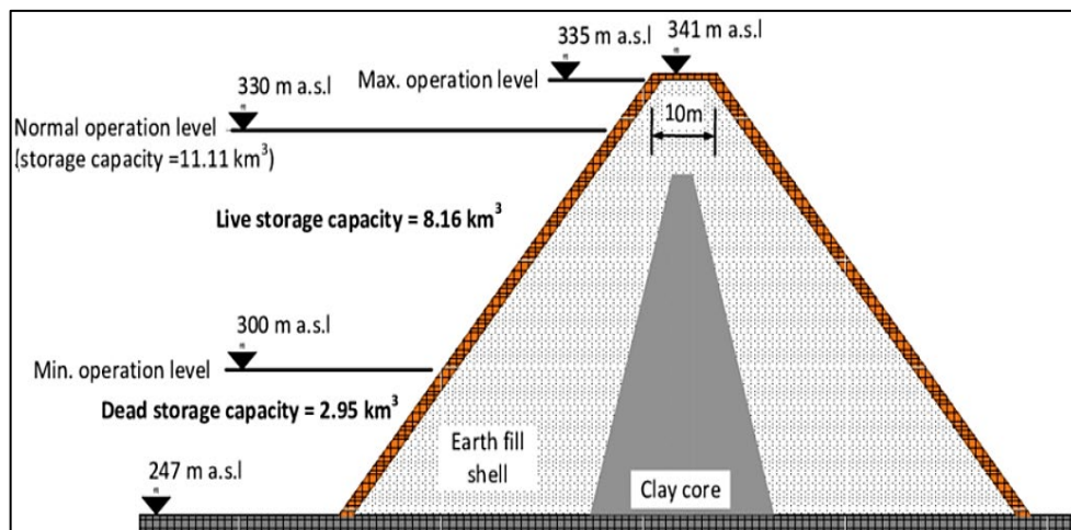
Figure 1: Cross section of Mosul dam [13]
