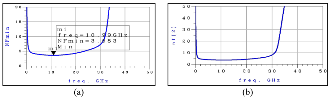
Figure 8: (a) The minimum NF of the proposed MQDDA. (b) The actual NF of the proposed MQDDA
