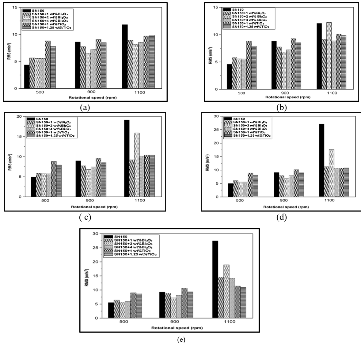
Figure 10: Optimum concentrations of Bi_2O_3 and TiO_2 blended with SN150 at various rotational speeds and dynamic loads of: (a) balanced system, (b) unbalanced system ( r_u=24 mm), (c) unbalanced system ( r_u=48 mm), (d) unbalanced system ( r_u=72 mm), and (e) unbalanced system ( r_u=96 mm)
