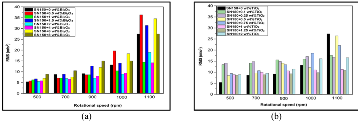
Figure 9: Variation of RMS with different rotational speeds and concentrations of nano additives at an unbalanced system ( r_u=96 mm): (a) SN150+ Bi_2O_3 and (b) SN150+ TiO_2
