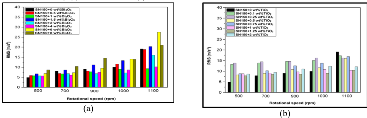
Figure 7: Variation of RMS with different rotational speeds and concentrations of nano additives at an unbalanced system ( r_u=48 mm): (a) SN150+ \text{Bi}_2\text{O}_3 and (b) SN150+ \text{TiO}_2
