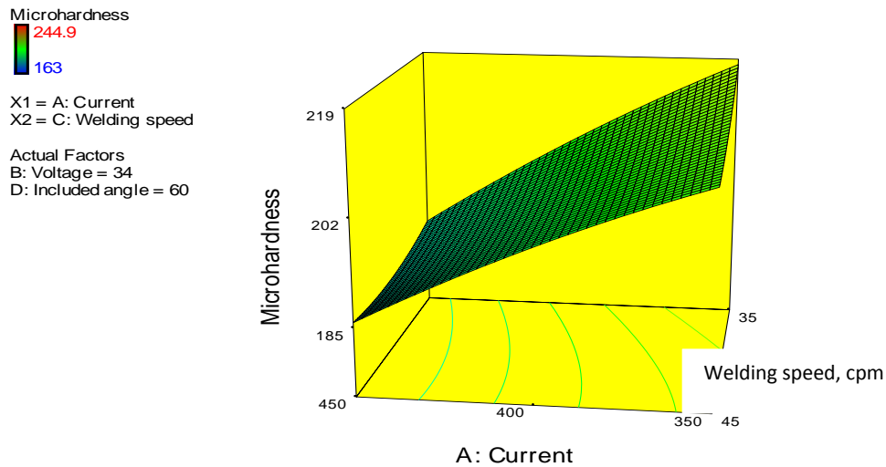
Figure 11: Minimum microhardness value at the optimum onditions (included angle of 60°, welding speed of 38 cpm, current of 450 amp, and voltage of 34 v)
