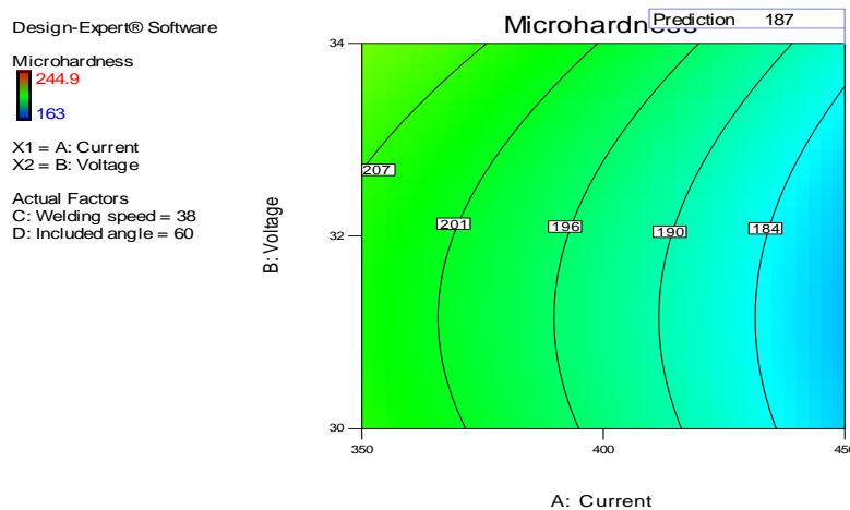
Figure 10: The lowest value of microhardness at the optimal conditions (included angle of 60°, welding speed of 38 cpm, current of 450 amp, and voltage of 34 v)
