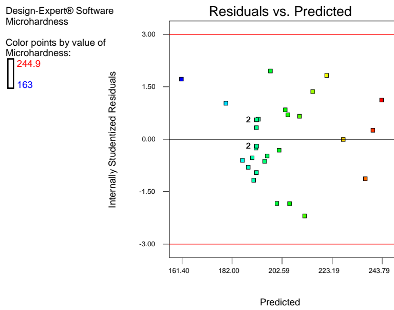
Figure 5: The residual against the predicted outputs for microhardness data.
