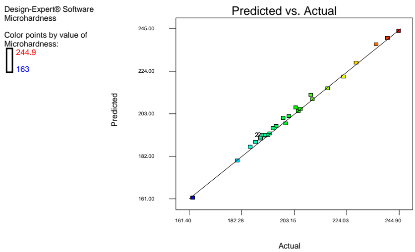
Figure 6: Predicted vs. actual microhardness results for comparison.
