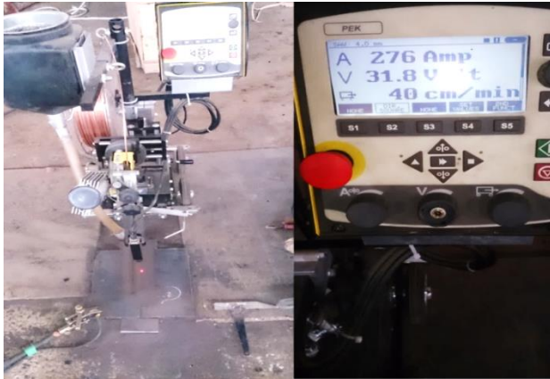
Figure 2: A view of EsabA2 Multitrack welding machine with the A2-A6 process controller PEK
