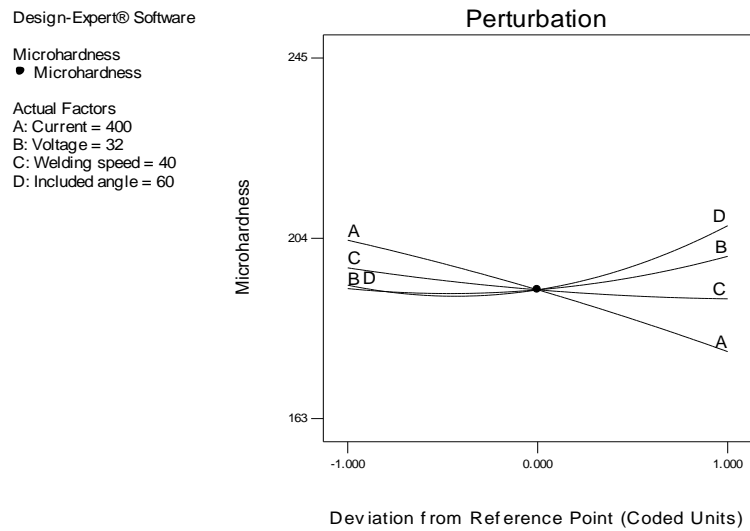
Figure 7: The microhardness perturbation depicting influence of every input factor along the chosen range.
