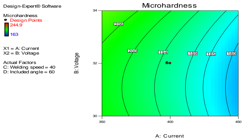
Figure 8: Two-dimensional plot of microhardness in terms of voltage and current at the center level ((60°) included angle and (40 cpm) welding speed).
