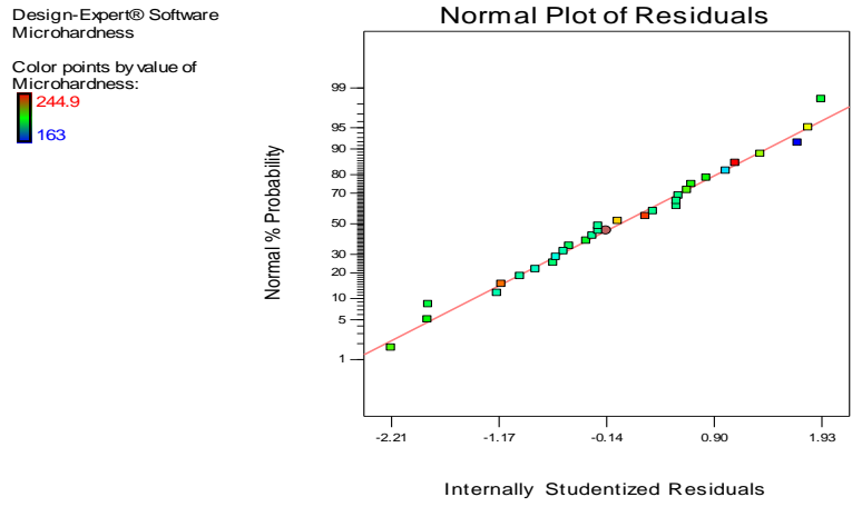
Figure 4: The normal probability of microhardness data
