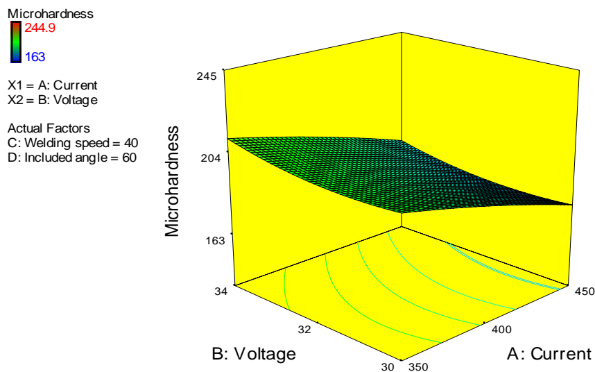
Figure 9: Three-dimensional plot of microhardness in terms of voltage and current at the center level ((60°) included angle and (40 cpm) welding speed).
