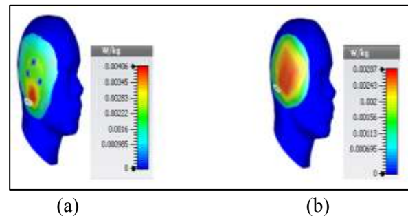
Figure 9: Specific absorbing rate (SAR) for child's head (11 years)(a) 1g, (b) 10g
