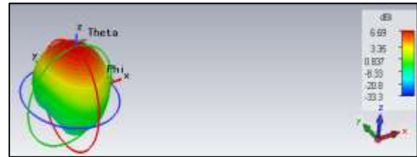
Figure 7: Directivity (dBi) for SPA at (2.4 GHz) for adult's head
