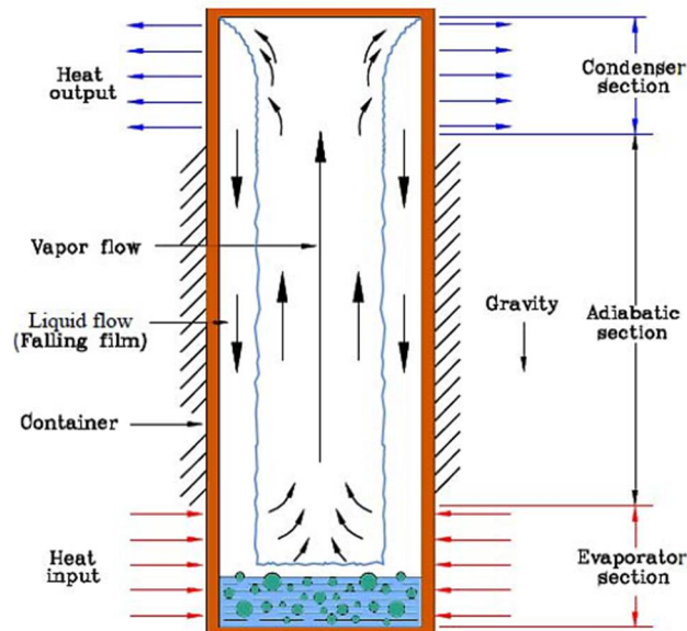
Figure 1: The schematic process of the Thermosyphon device
