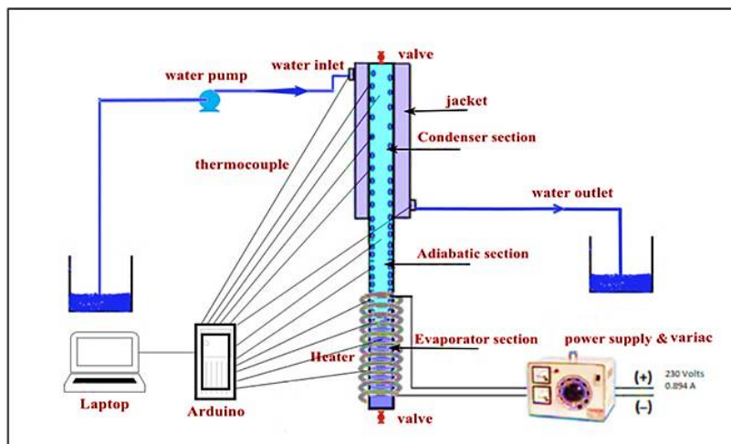
Figure 3: A schematic diagram of the test rig
