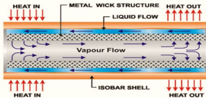
Figure 2: Conventional heat pipe
