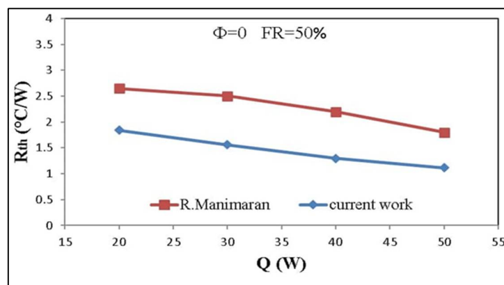
Figure 7: Comparison results of thermal resistance vs. heat inputs of the present work and R. Manimaran [5]
