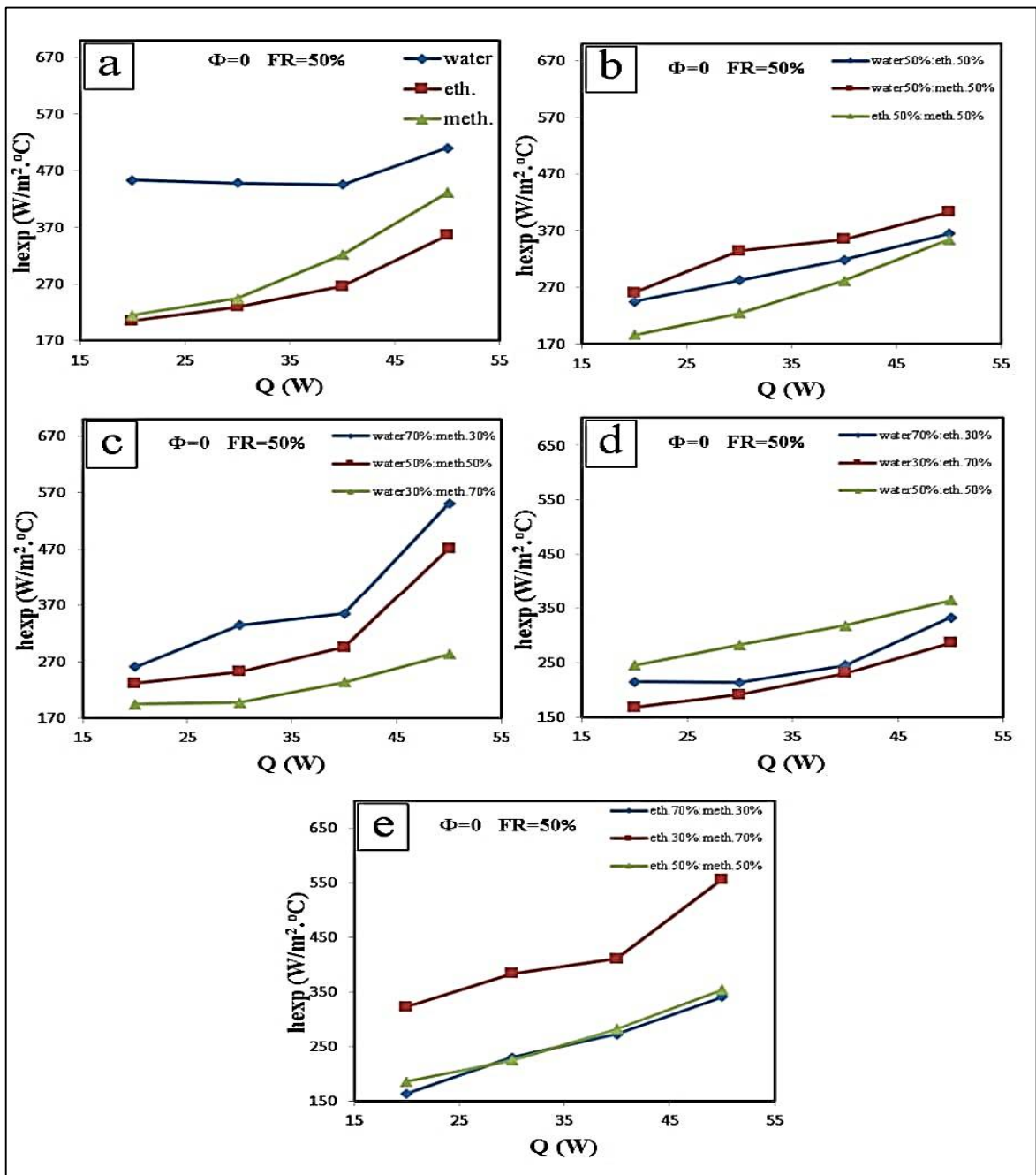
Figure 6: Heat transfer coefficient vs. heat input using: (a) pure working fluids, (b) binary fluids with (50:50) % mixing ratio, (c) binary fluids water&Methanol, (d) binary fluids water & ethanol, and (e) binary fluid ethanol & Methanol
