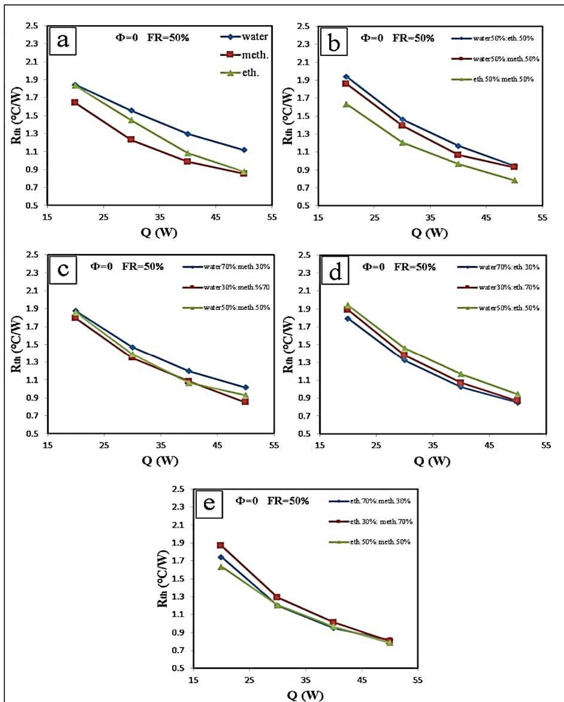
Figure 5: Thermal resistance vs. heat input using: (a) pure working fluids, (b) binary fluids with (50%: 50%) mixing ratio, (c) binary fluids water& Methanol, (d) binary fluids water & ethanol, and (e) binary fluid ethanol & Methanol
