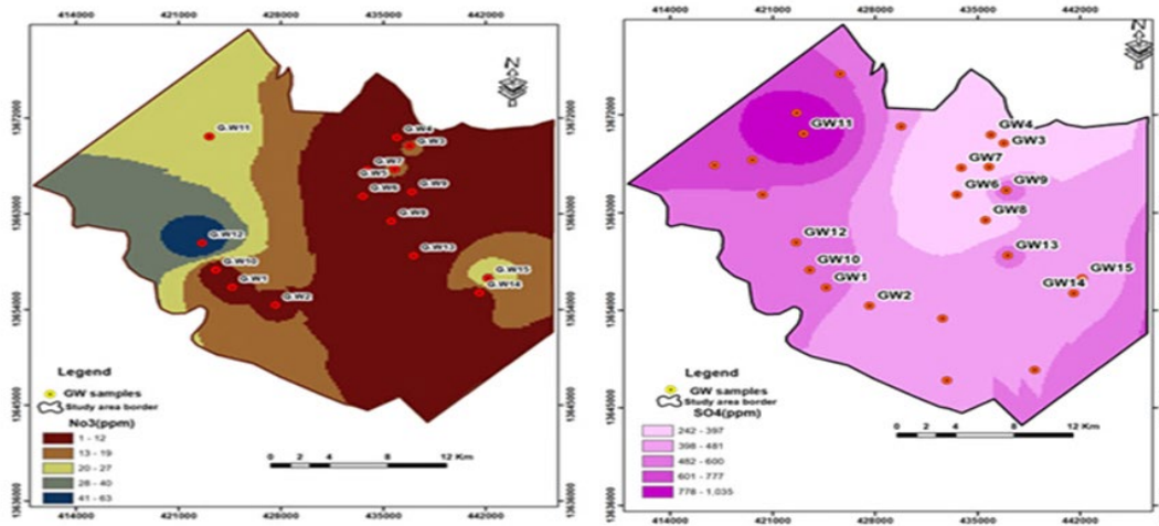
Figure 6: Spatial distribution of concentration in the study area (I) NO_3^- (J) SO_4^{2-}
