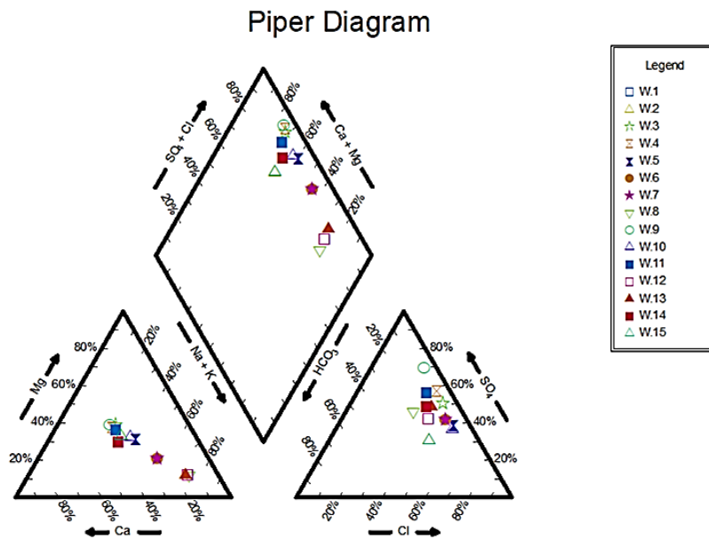
Figure 9: Piper diagram of the water tests in the study area
