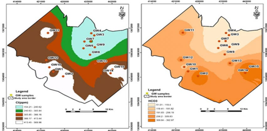
Figure 5: spatial distribution of concentration in the study area (G) Cl^{-} (H) HCO_3^{-}
