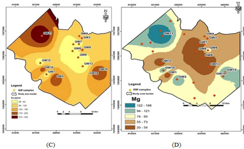
Figure 3: spatial distribution for concentrations in research area (C) Ca^{+2} (D) Mg^{+2}
