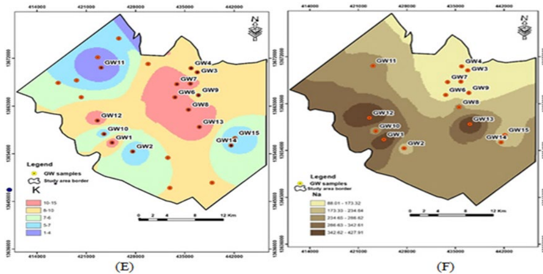
Figure 4: Spatial distribution of concentration in the study area (E) K^{+} (F) Na^{+2}
