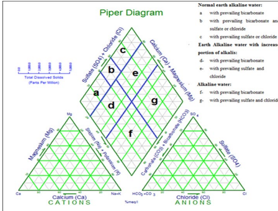
Figure 8: Standards plotting of Piper trilinear diagram, (1944) with the divisions of Langguth, (1966)
