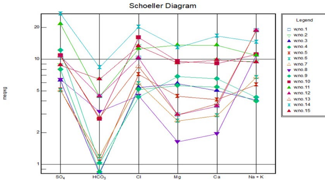
Figure 11: Schoeller's classification (1972) of the water in the study area
