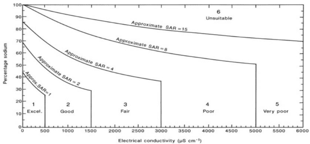
Figure 12: USDA classification [13]
