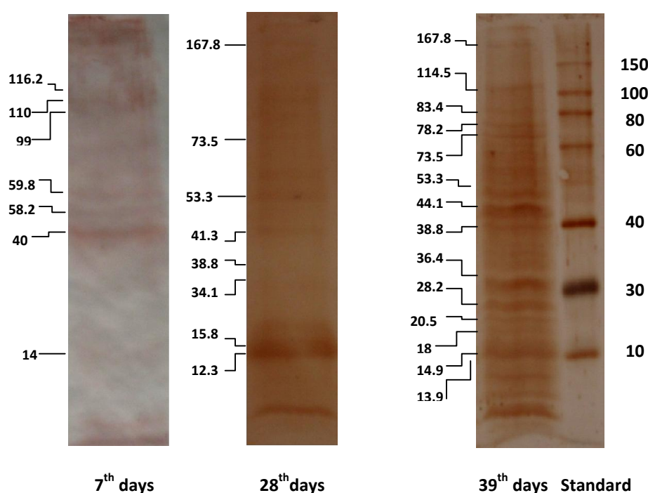
Picture(3): Immunoblot of proteins transferred from a 5-15 %SDS-PAGE. Lanes are immunoblots of Oocyst extract preparations probed with immune serum (7 th days) :after first dose of vaccine ; (28 th days): after second dose of vaccine and (39 th days) after challenge with E.tenella oocysts.
