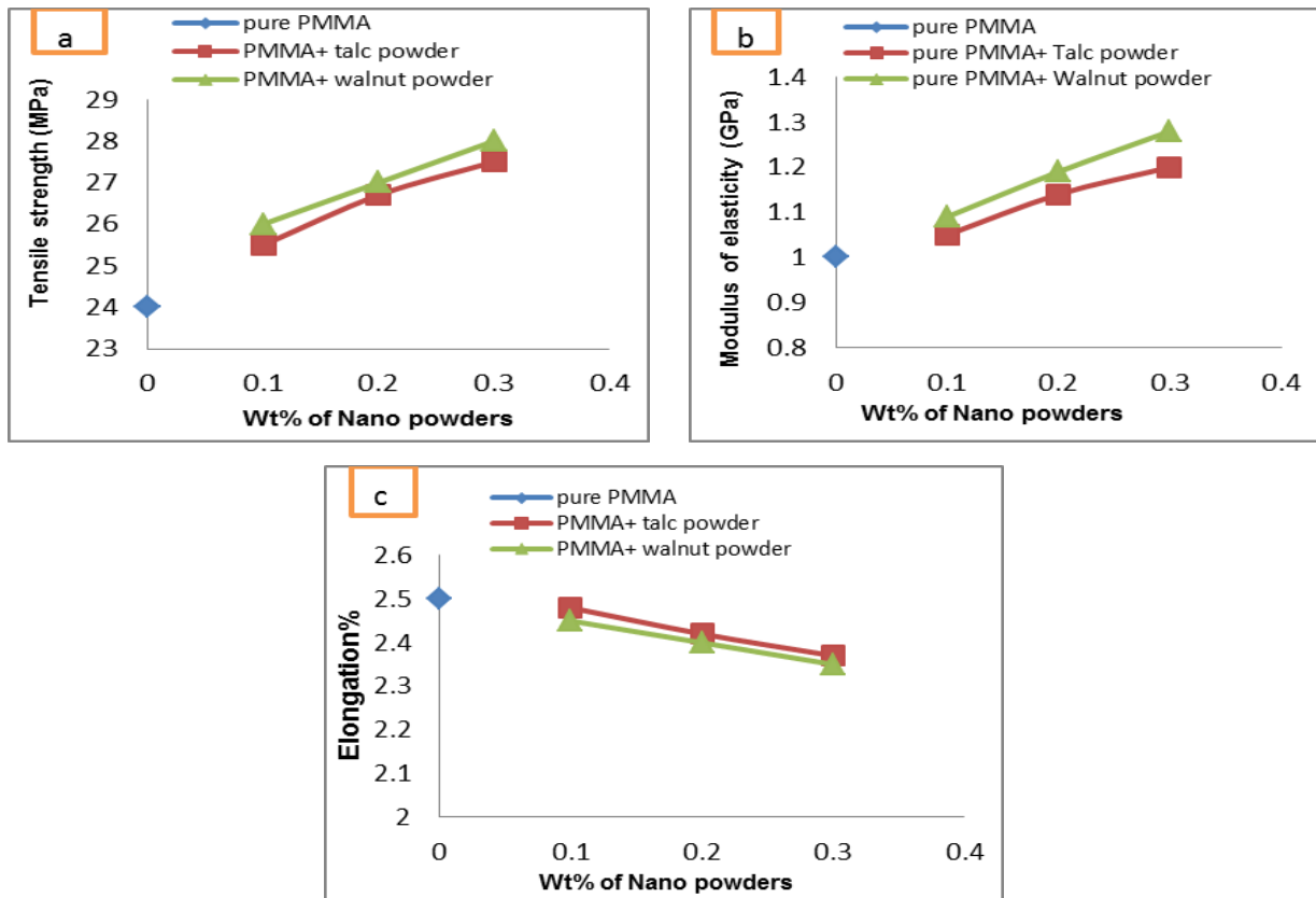
Figure 3: (a) Tensile Strength, (b) Modulus of Elasticity, and (c) Elongation at break of polymer Nano composite (PMMA: X% Nanoparticles) as a component of (WSP and TP) particles
