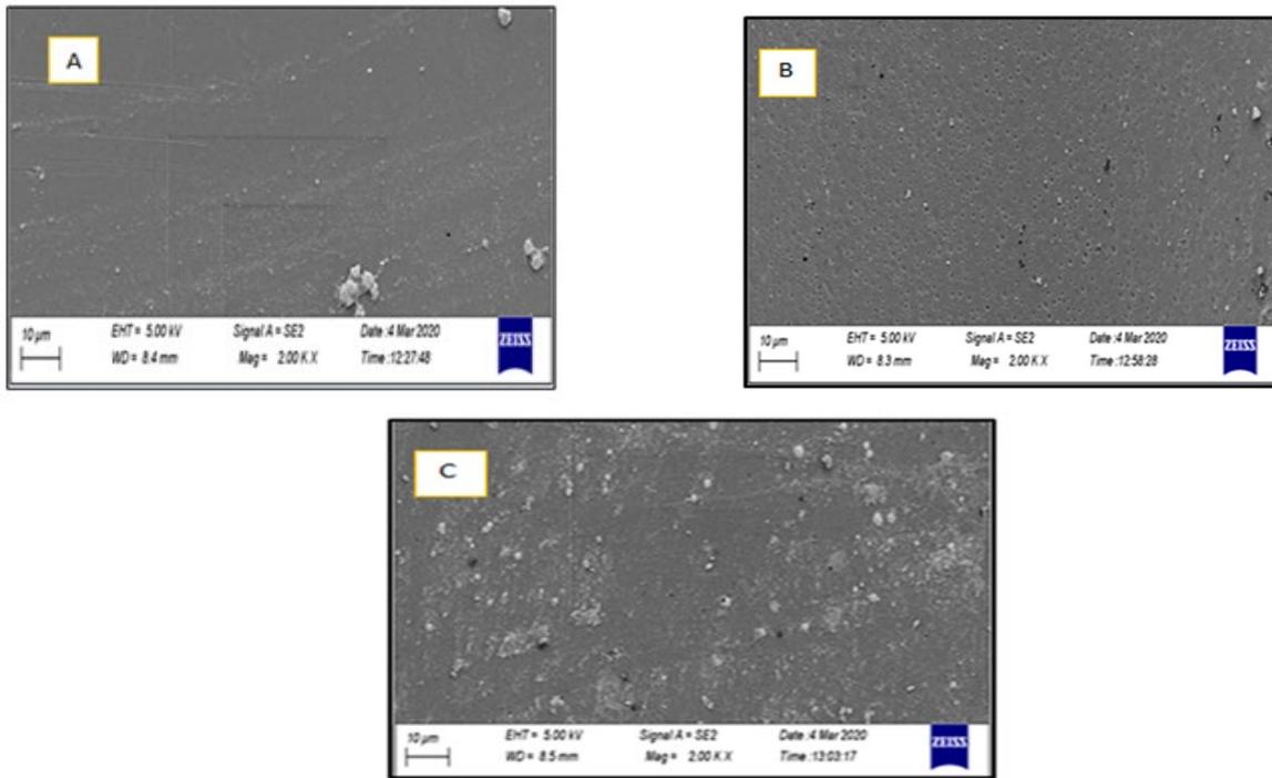
Figure 5: The Morphology of Surface for (a): pure acrylic resin (PMMA), (b) for polymer Nano composite (PMMA: 0.3% WSP) and (c) for polymer Nano composite (PMMA: 0.3% TP) at magnification (x2000)
