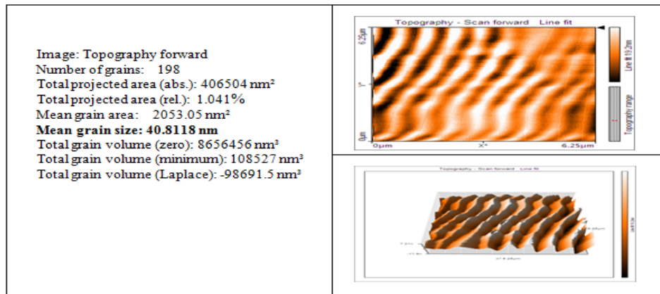
Figure 1: Illustrates the AFM test of Walnut shell nanoparticles
