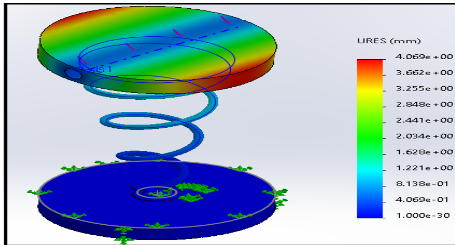
Figure 8: The deformation distributed in the head of spring
