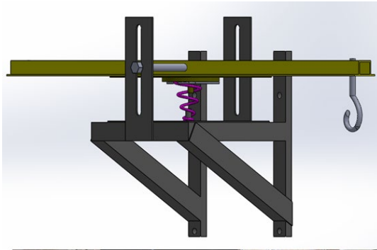
Figure 3: lateral stiffness testing system
