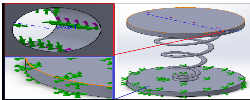
Figure 5: The boundary condition (the green color) and the moment applied (the purple color)
