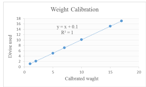
Figure 7: Weight calibration relationship
