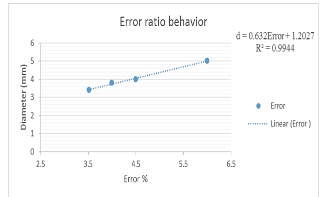
Figure 12: Diameter- error ratio relationship
