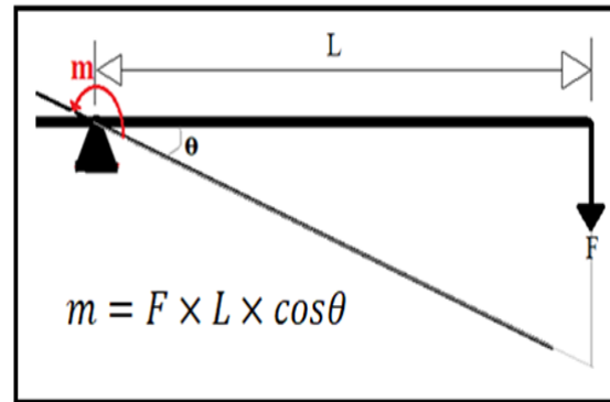
Figure 4: The process of converting force into the moment (force application method)
