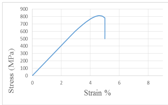
Figure 6: Stress-Strain curve for the used wire
