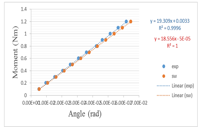
Figure 10: Moment-Angle relationship for 3.8 mm conical spring
