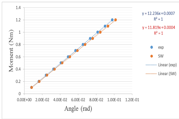
Figure 9: Moment-Angle relationship for 3.4 mm conical spring
