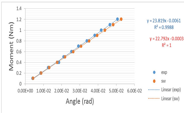
Figure 11: Moment-Angle relationship for 5 mm conical spring
