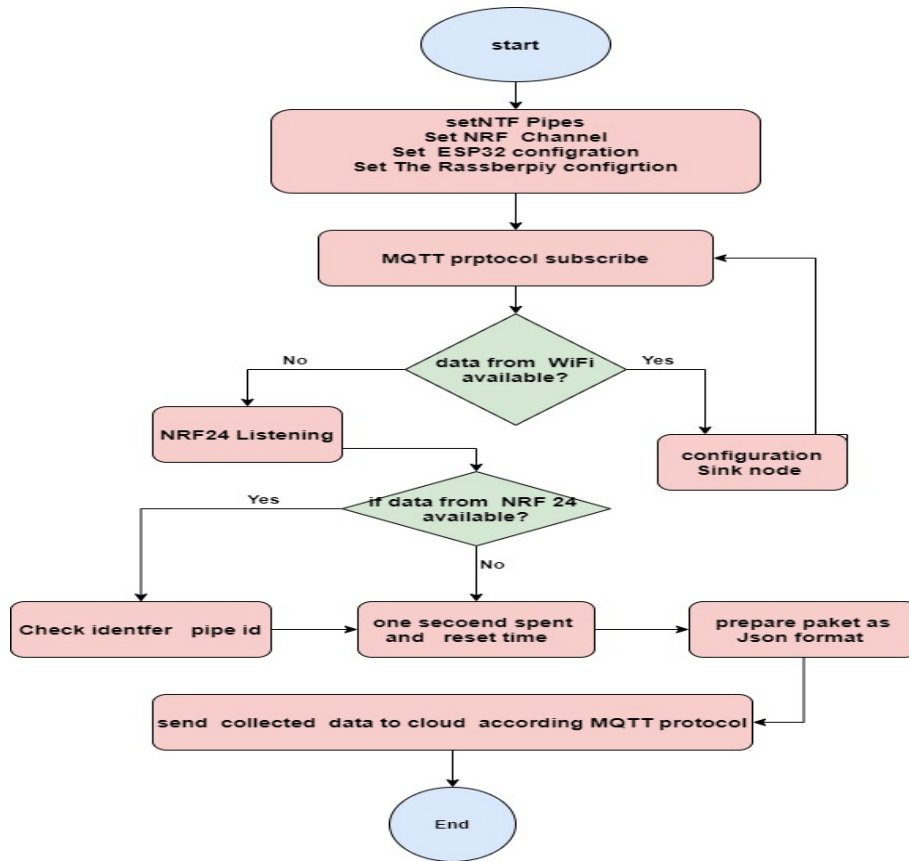
Figure 3: The proposed algorithm of the sink node
