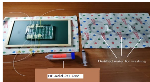
Figure 3: Chemical Etching
