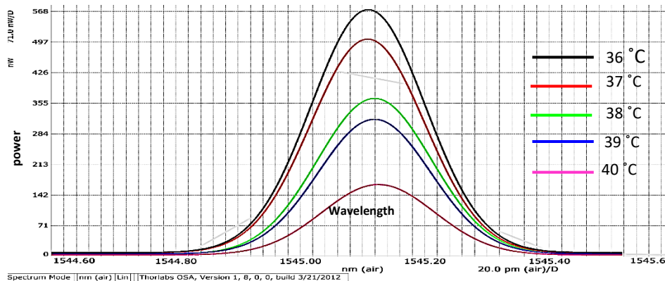
Figure 4: The transmission spectra of the optical signal propagated along with the Single-mode fiber with a diameter 125 µm for the temperature sensor
