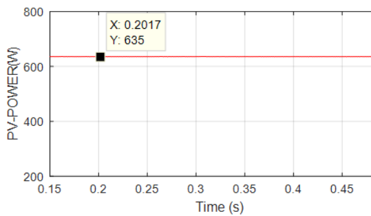
Figure 9: P_{pv} @ 400W/ m 2 , 25°C R_L (200Ω)
