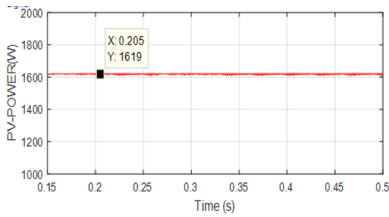
Figure 3: P_{pv} @ 1000W/ m 2 , 25°C R_L (50Ω)
