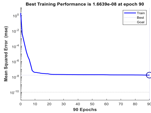
Figure 10: The training performance of ANN error
