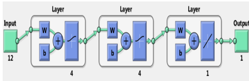
Figure 8: The applied neural network with two hidden layers
