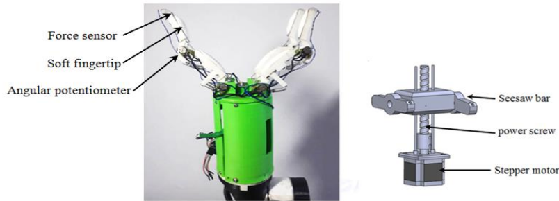
Figure 1: The under-actuated robotic hand with linkage seesaw differentials
