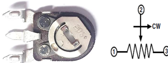
Figure 3: Angular potentiometer with Circuit diagram of potentiometer
