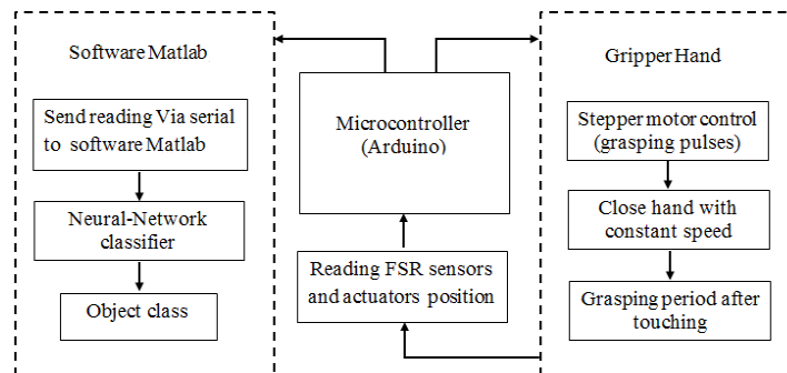
Figure 7: The block diagram of the data acquisition method with software program for classification objects
