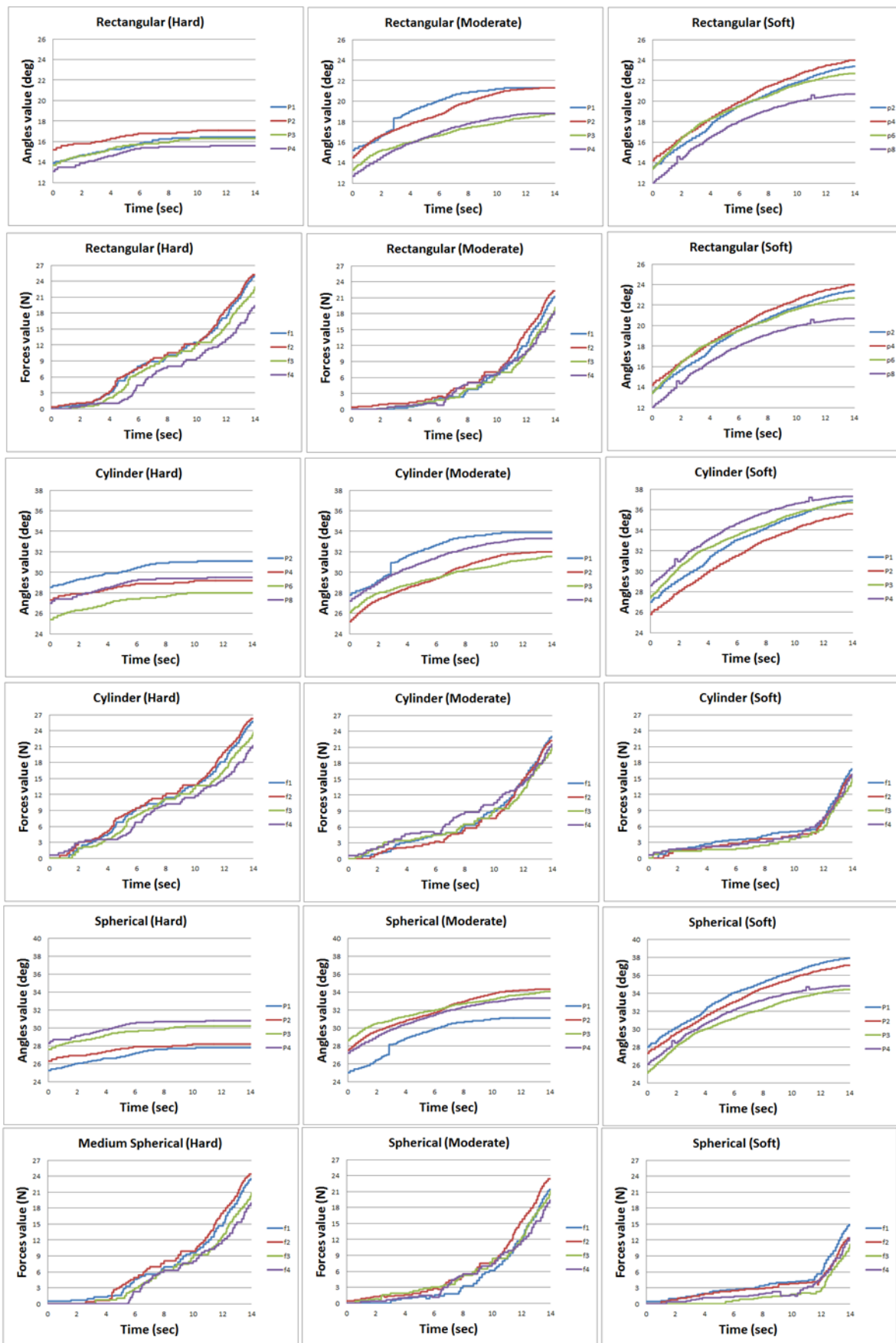
Figure 9: The force and actuator data resulting during grasping of rectangular, cylinder and spherical objects with three different softness at time series response.
