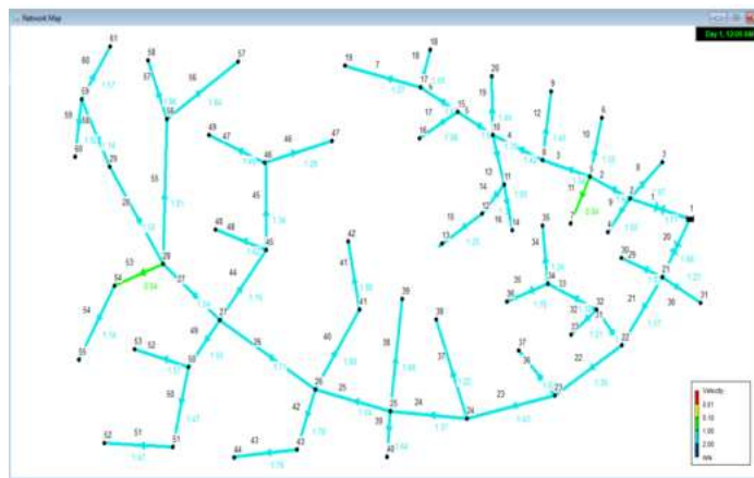
Figure 4: Velocity distribution along the pipeline in the irrigation project
