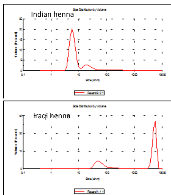
Figure 5: shows the size distribution of silver nanoparticles prepared by different types of henna.
