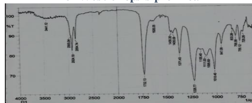
Figure 2: FTIR spectral of Crude extracellular extract of W. Prolifica
