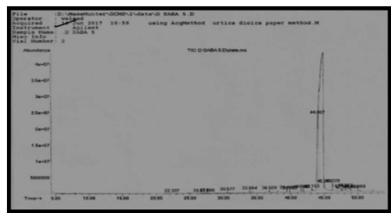
Figure 6: GC- Mass analysis of extracellular extracts in Group2 (Benzene 50 ml)
