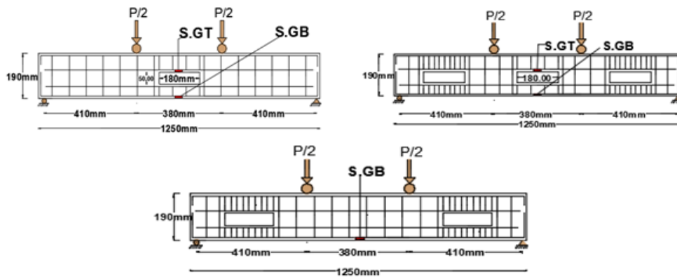
where S.GT-strain gage at Top, S.GB-strain gage at Bottom
