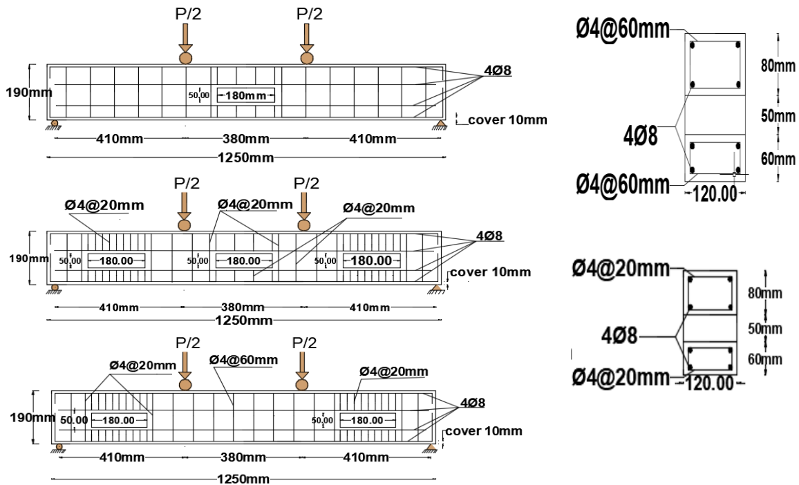
Fig. 2. The beams details.
