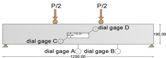
Fig. 3. Location of the dial gauge at beams.
