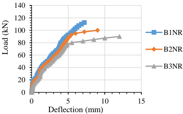
Fig. 9. Effect number of openings on load-deflection for NR at mid-span.
