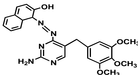
1-[2-Amino-5-(3,4,5-trimethoxy-benzyl)-pyrimidinyl-4-azo]-1,8a-dihydro-naphthalene-2-ol
