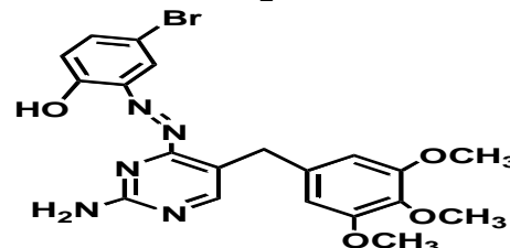
2-[2-Amino-5-(3,4,5-trimethoxy-benzyl)-pyrimidinyl-4-azo]-4-bromo-phenol
