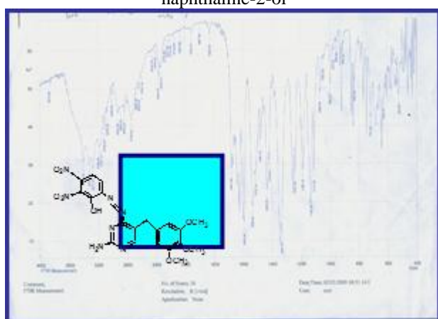
Figure (2) FT-IR spectrum of 6-[2-Amino-5-(3,4,5-trimethoxy-benzyl)-pyrimidinyl-4-azo]-2,3-dinitro-phenol.
