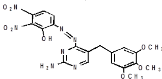
6-[2-Amino-5-(3,4,5-trimethoxy-benzyl)-pyrimidinyl-4-azo]-2,3-dinitro-phenol
