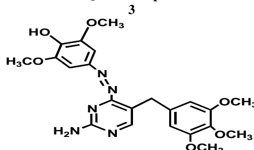
4-[2-Amino-5-(3,4,5-trimethoxy-benzyl)-pyrimidinyl-4-azo]-2,6-dimethoxy-phenol
