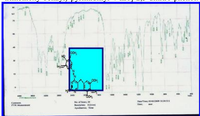
Figure (3) IR spectrum of 4-[γ-Amino-5-(3,4,5-trimethoxy-benzyl)-pyrimidinyl-ε-azo]-2,6-dimethoxy-phenol.
