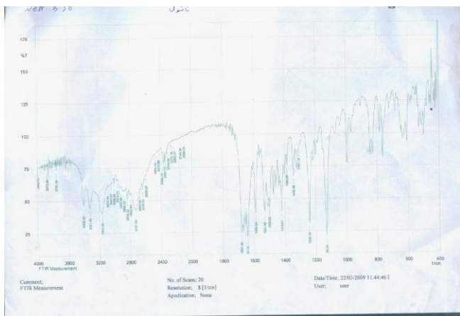
Figure (1) FT-IR spectrum of 1-[2-Amino-5-(3,4,5-trimethoxy-benzyl)-pyrimidinyl-4-azo]-1,8a-dihydro-naphthaline-2-ol
