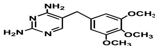
5-(3,4,5-Trimethoxy-benzyl)-pyrimidine-2,4-diamine (Trimethoprim)
