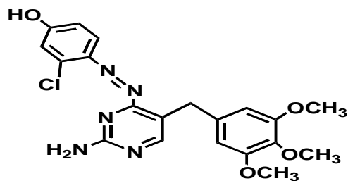
4-[2-Amino-5-(3,4,5-trimethoxy-benzyl)-pyrimidinyl-4-azo]-3-chloro-phenol
