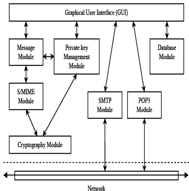
Fig. 4: Secure E-mail Client Architecture.
