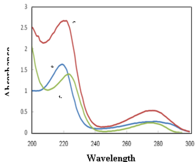
Fig. 1. Absorption (zero-order) UV spectra of (a) 10.0 µg ml -1 tryptophan, (b) 40.0 µg ml -1 tyrosine, (c) mixture of 10.0 µg ml -1 tryptophan and 40.0 µg ml -1 tyrosine, in distilled water.
