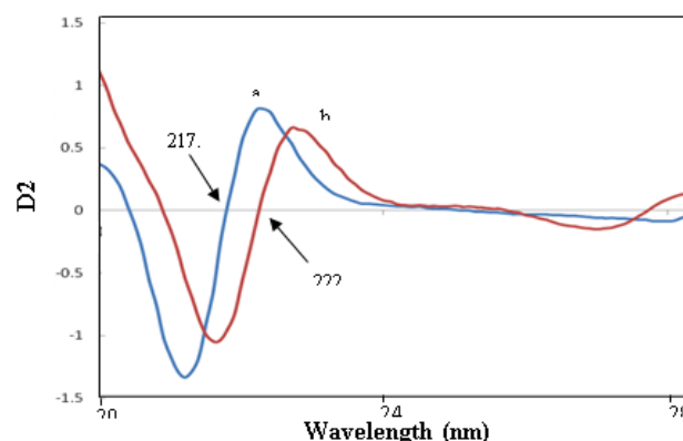
Fig. 2. Differential-derivative spectra of (a) 10.0 µg ml -1 tryptophan, (b) 40.0 µg ml -1 tyrosine in distilled water.
