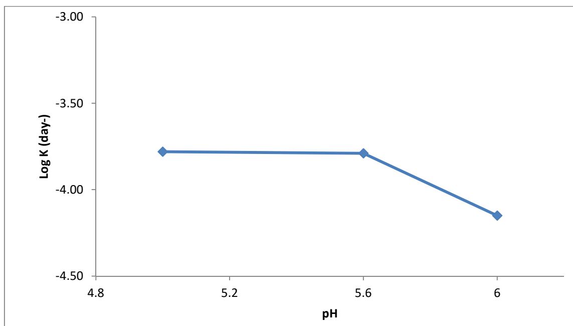
Figure 4: pH-degradation rate of gatifloxacin solution in phosphate buffer for formula 15,16 and 17 at pH range (5.0-6.0) and 0.25 ionic strength at 60°C.
