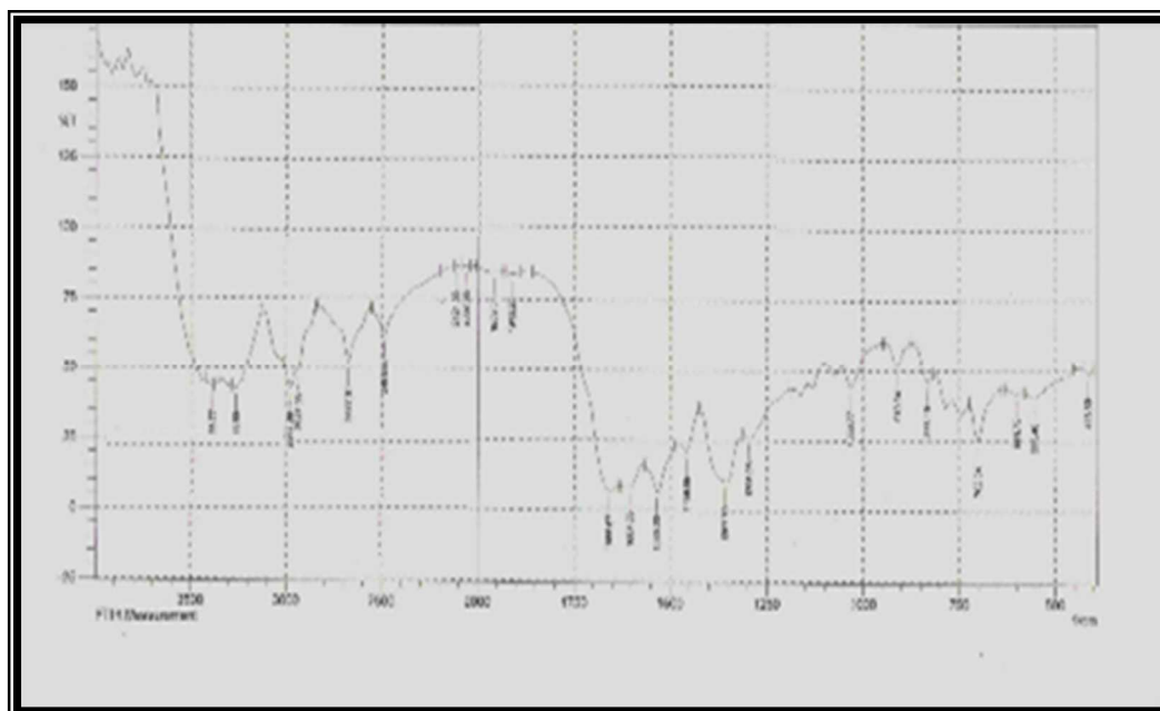
Fig. ( 4 ) FT-IR spectra of compound ( 7 )
