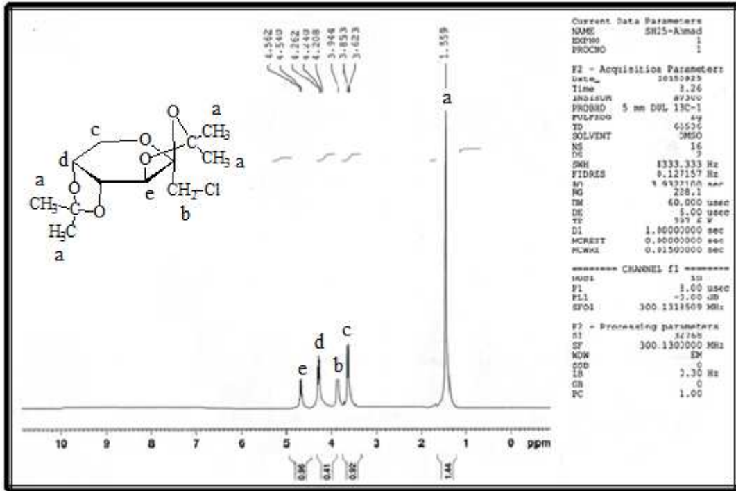
Fig. ( 1 ) H-NMR spectra of compound ( 9 )
