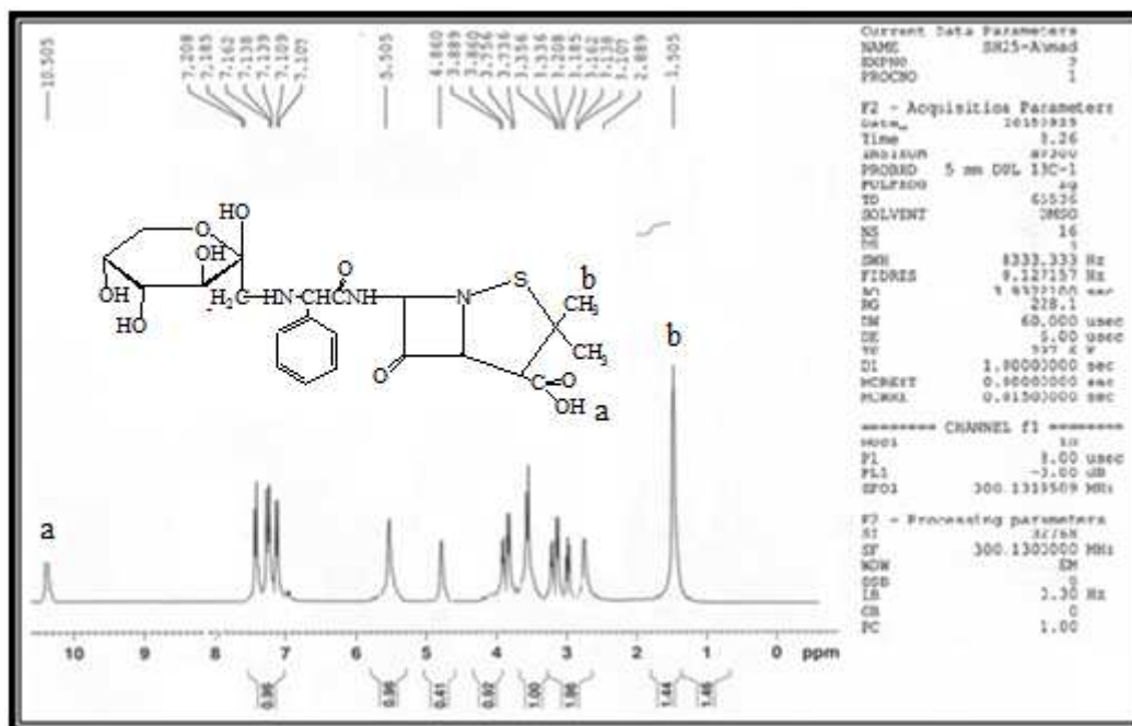
Fig. ( 3 ) 1 H-NMR spectra of compound ( 7 )
