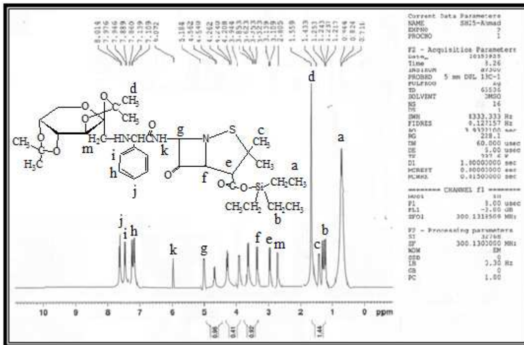
Fig. (2) H-NMR spectra of compound (10)
