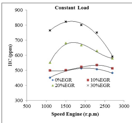
Fig. 6. EGR effect on HC concentrations at variable engine speeds and constant load
