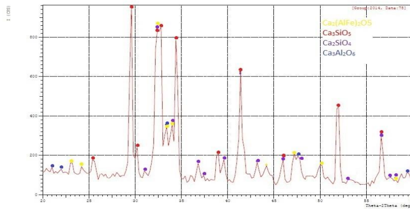
Figure (3) The XRD Spectra of cement powder
