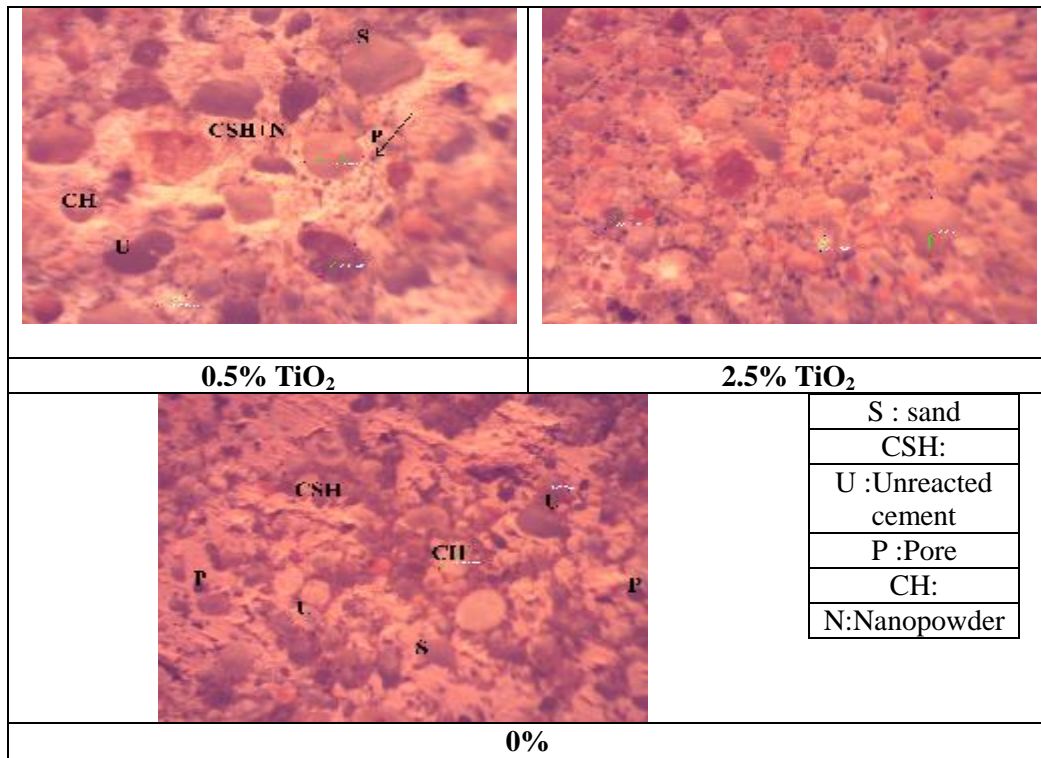
Figure (5) Optical microscopy image for TiO 2
