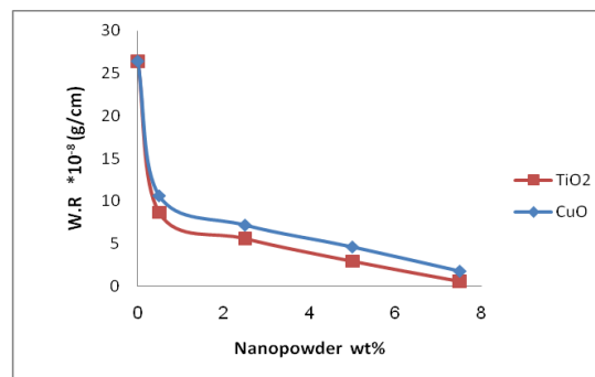
Figure (10) Wear rate of prepared mortar at different weight ratio.
