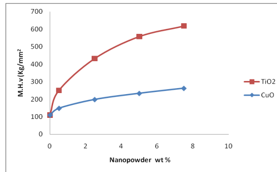
Figure(9) Microhardness of prepared mortar at different weight ratio.
