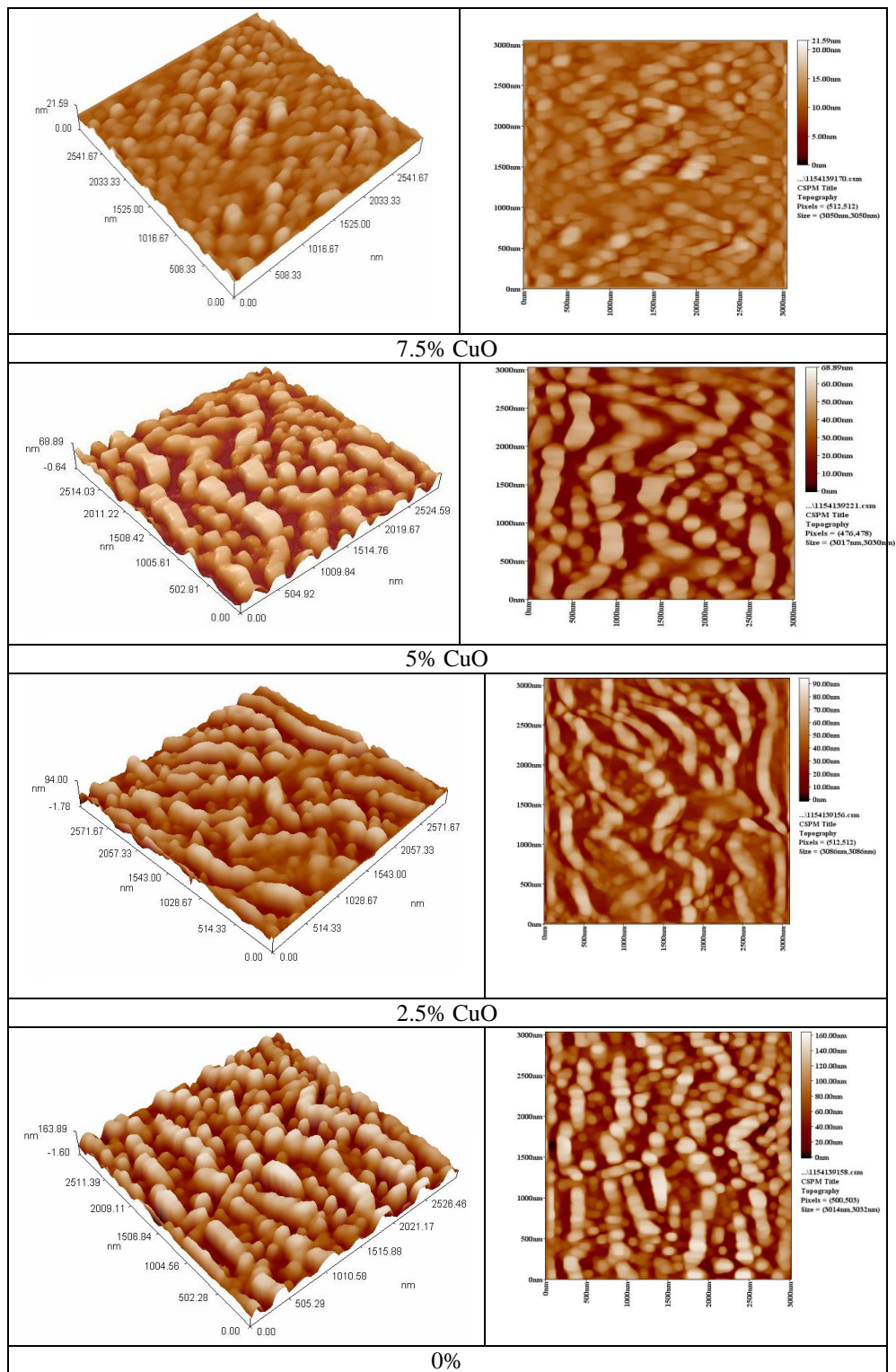
Figure (8) 3-D AFM images of the Mortar mixed CuO at different ratio.
