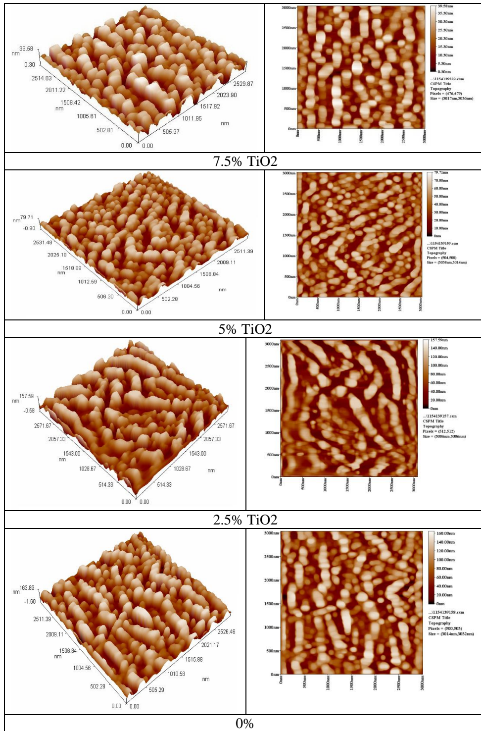
Figure (7) 3-D AFM images of the Mortar mixed TiO 2 at different ratio.
