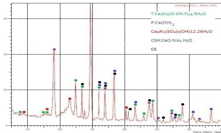
Figure (3) The XRD Spectra of cement powder
