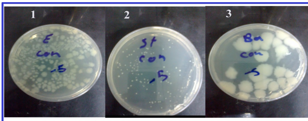
Figure (7).(1) Escherichia coli bacteria with control before growth 20 \times 10^7 cell / ml (2) Staphylococcus aurius bacteria with control before growth 11.3 \times 10^7 cell / ml (3) Bacillus cereus bacteria with control growth before 2.5 \times 10^7 cells / ml.
