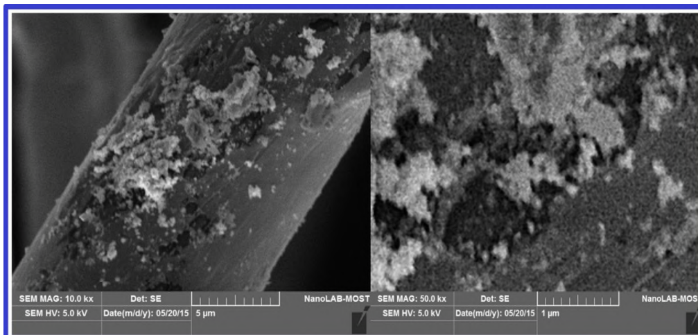
Figure (5) SEM images of antibacterial CuO –TiO 2 –ZnO thin films coated cotton fabric.
