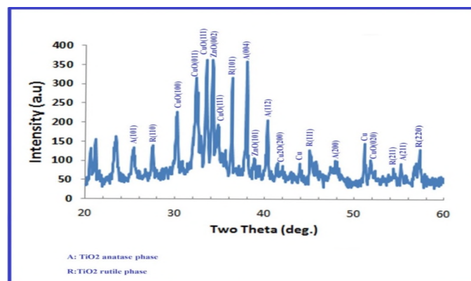
Figure(3) XRD patterns of CuO-TiO 2 - ZnO mixture.
