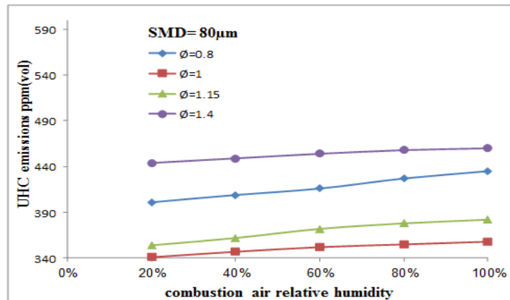
Figure (9) UHC emission with increasing inlet air humidity at different equivalence ratio
