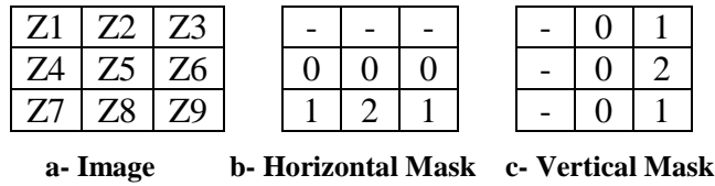
Figure (10): Sobel Masks.
