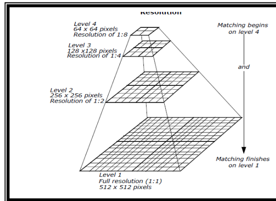
Figure (3): Image Pyramid for Matching at Coarse to Full Resolution Triangulation
