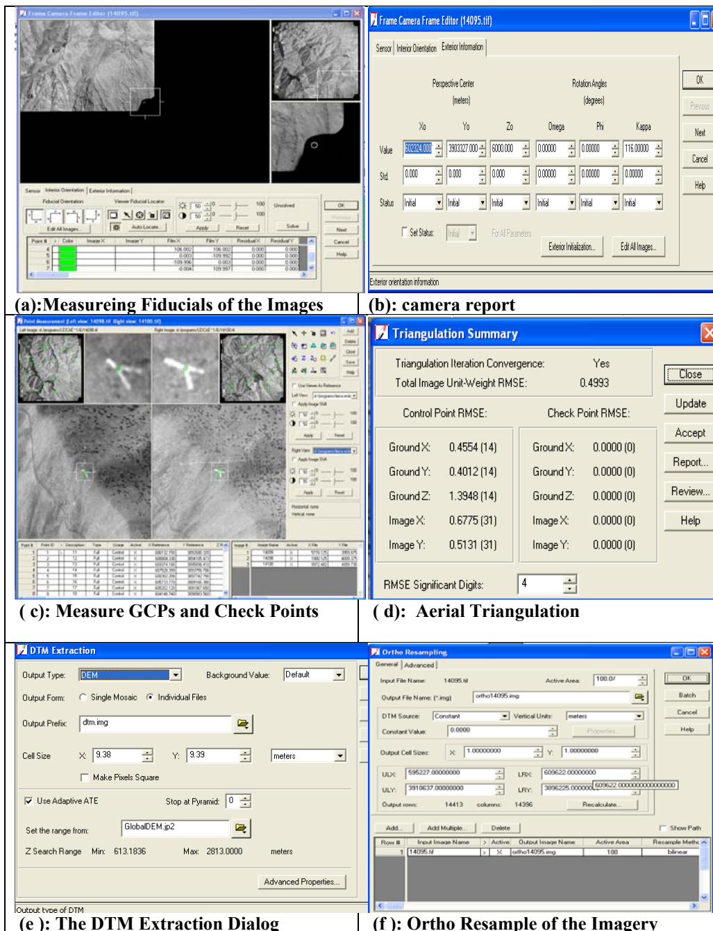
Figure (6): Steps of DTM extraction by ERDAS Imagine.
