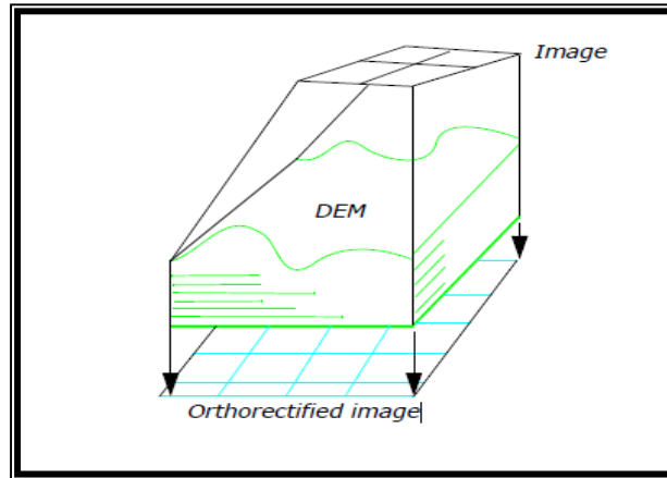
Figure(4): Orthorectification
