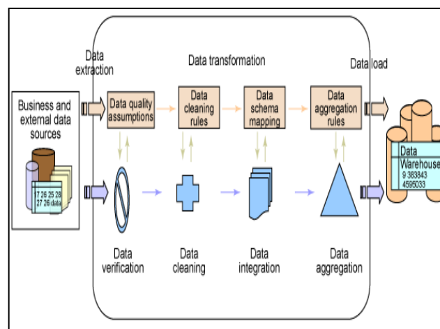
Fig.1 ETL Process.
