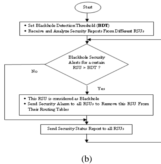
Fig. 8 The suggested anti-black hole attack IDS procedure (a)RSU side (b) VANET server side
