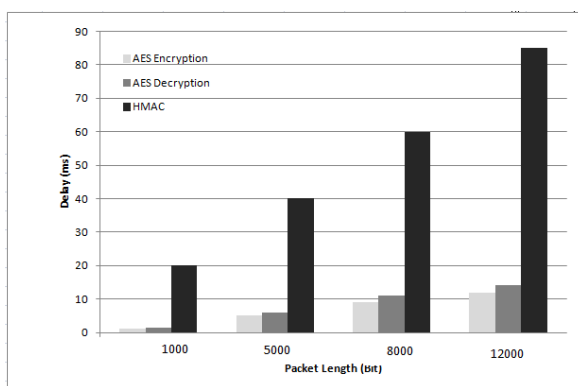
Fig. 13 Ubicom's performance for AES encryption/decryption and HMAC (SHA2) for different packet lengths
