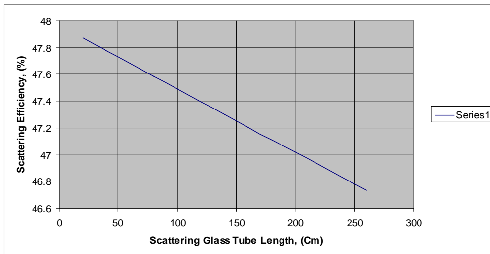
Figure (12) Scattering glass tube efficiency versus its length.
