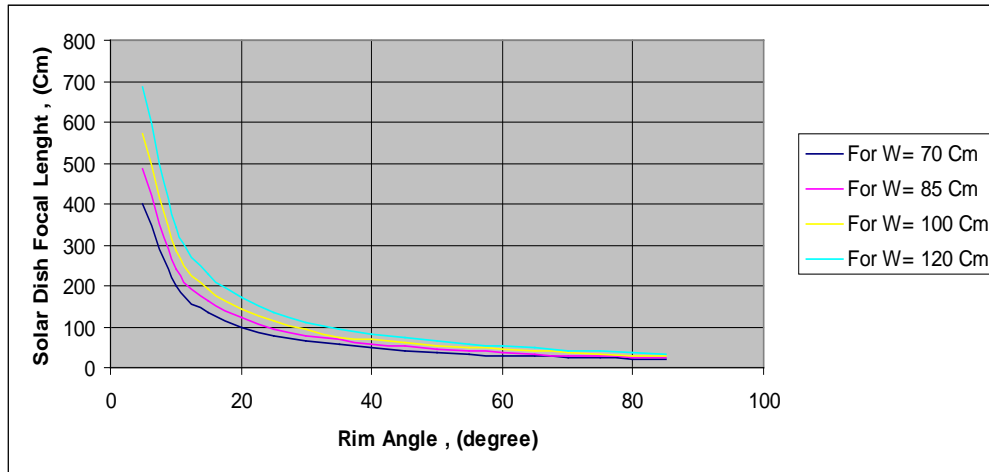
Figure (5) Solar dish's focal lengths versus rim angles for different aperture diameters.
