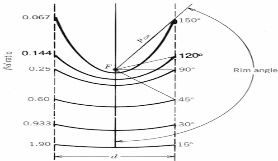
Figure (2) Shows primary reflector (dish) geometrical dimensions [14].
