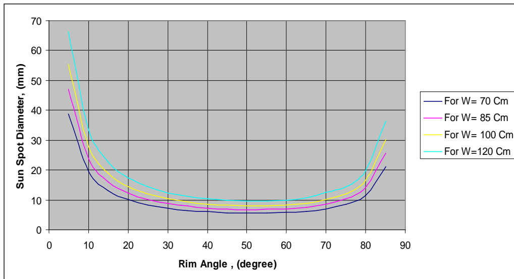
Figure (6) Sun's spot diameter versus rim angles for different aperture diameters.
