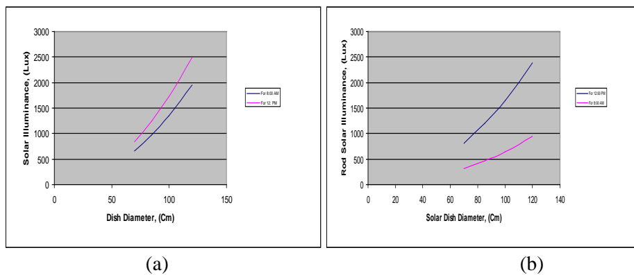
Figure (12) Shows scattered visible solar illuminance from the glass rod versus dish diameter for (a) 21 June (b) 21 December.
