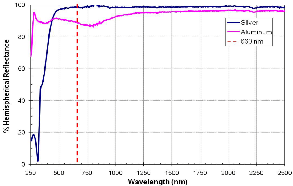
Figure (9) Comparison curve for reflection between solar dish's surface area coating by Silver and Aluminum versus solar spectrum wavelengths.
