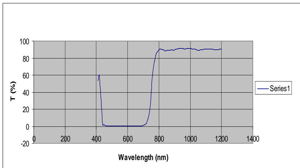
Figure (10) Transmission curve of sunlight versus wavelengths by using cold mirror.
