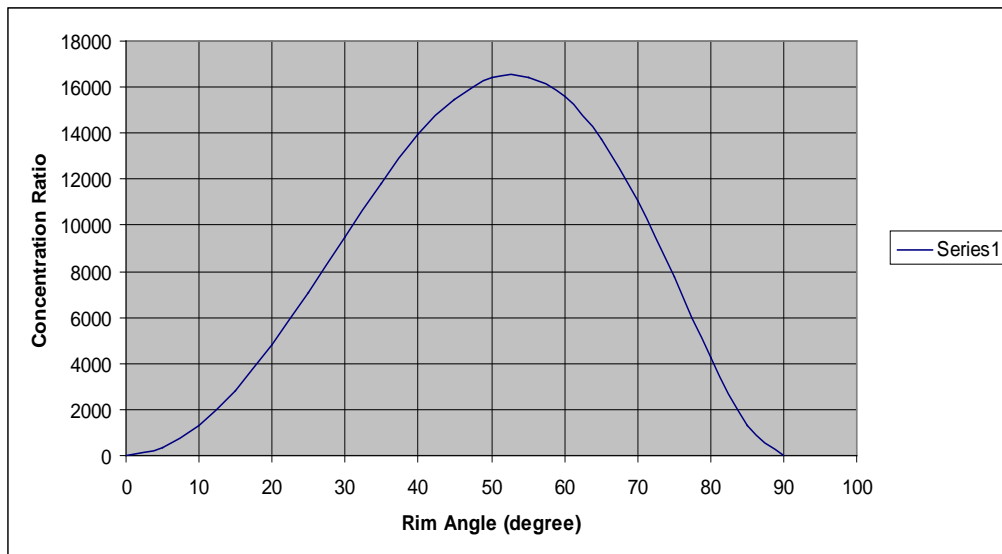
Figure (8) Solar dish's concentration ratio versus rim angles for different aperture diameters.
