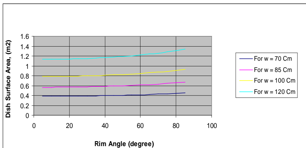
Figure (4) Solar dish's surface areas versus rim angles for different aperture diameters.
