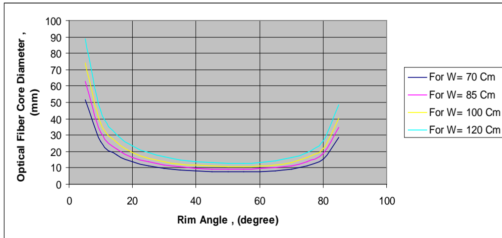
Figure (7) Plastic optical fiber diameter versus rim angles for different aperture diameters.
