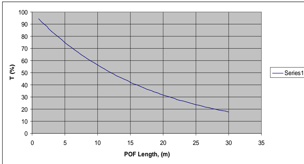
Figure (11) Plastic optical fiber transmission versus its length for visible sunlight spectrum.
