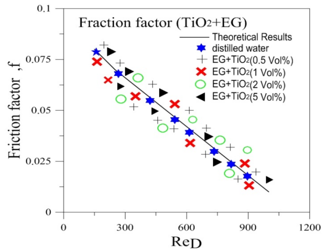
Figure (20) The friction factor of TiO 2 + EG nanofluid in fully developed laminar flow.
