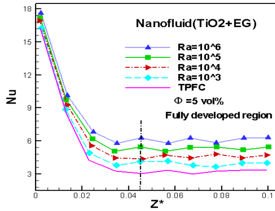
Figure (26) The local Nusselt number of TiO 2 + EG Nanofluid at \Phi = 5 vol % and different Ra.
