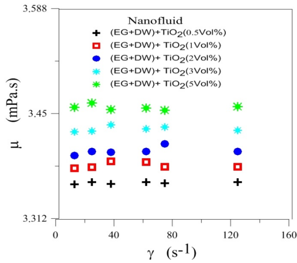
Figure (34) Viscosity as a function of shear rate for TiO 2 + (EG+DW) nanofluid.
