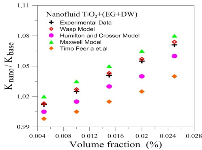
Figure (10) Thermal conductivity ratio for TiO 2 + (EG+DW).
