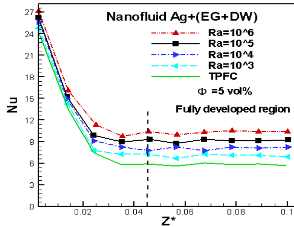
Figure (29) The local Nusselt number of Ag+(EG+DW) nanofluid at \Phi = 5 \text{ vol } \% and different Ra.
