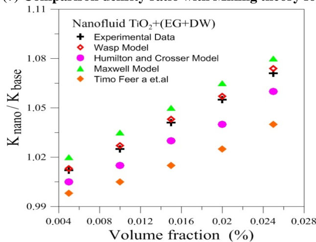
Figure (8) Comparison density ratio with mixing.
