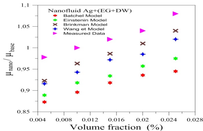
Figure (5) Viscosity ratio for Ag+ (EG+DW).
