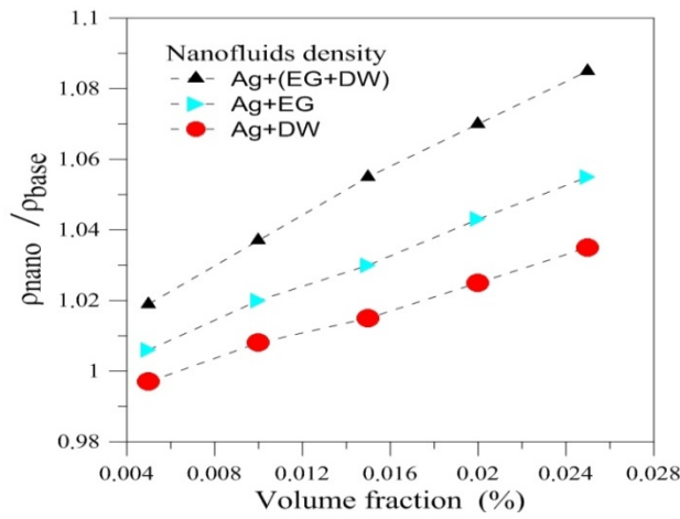
Figure (9) Three types of density ratio for Ag.
