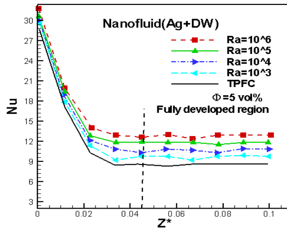
Figure (25) The local Nusselt number of Ag+ DW nanofluid at \Phi = 5 vol % and different Ra.
