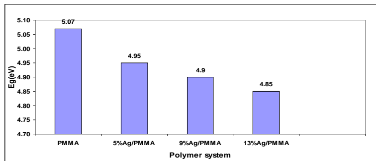
Figure (5) Energy gap values for for (PMMA), and (Ag/PMMA) composites at different concentration.
