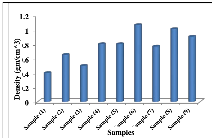
Figure (2) shown the density values of samples
